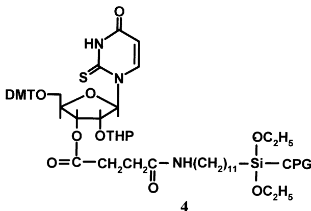
Figure 2. 2-Thiouridine derivative attached to leaa CPG.
