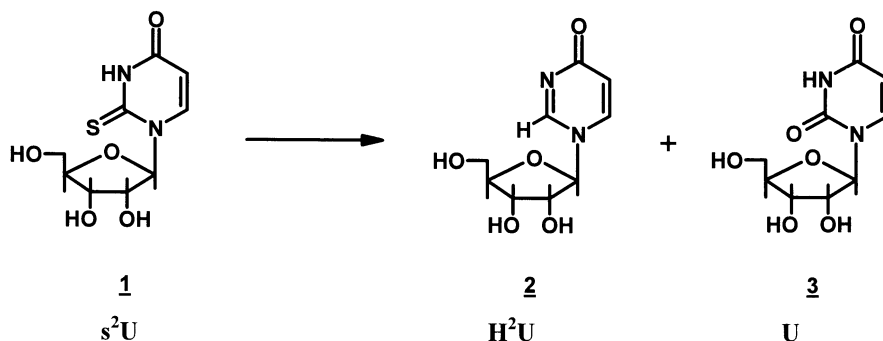
Figure 1. Products of 2-thiouridine oxidative desulfurization and oxidation.
