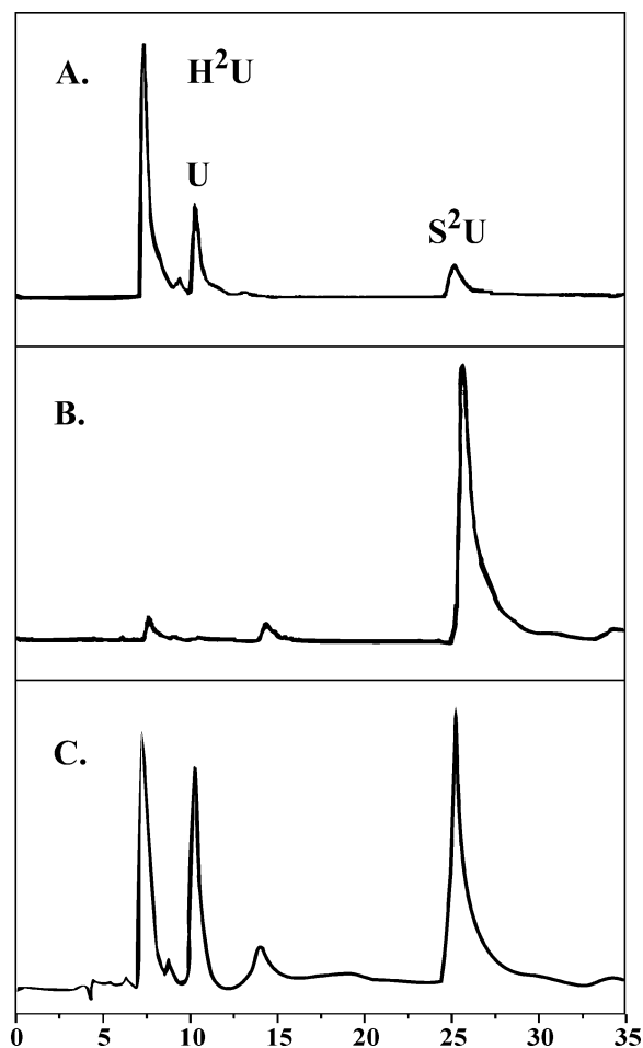
Figure 3. HPLC traces of: (A) equimolar mixture of H^2U , U and s^2U ; (B) the elution profile for the test that utilized CCl_4 /NMM oxidizer (entry 4, Table 1); (C) the elution profile for the test that utilized 1 M tBuOOH in methylene chloride as the oxidizer.
